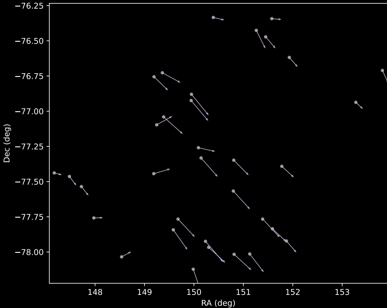
APOGEE DR17 Cluster 9 Proper Motion Vectors (n=34)
