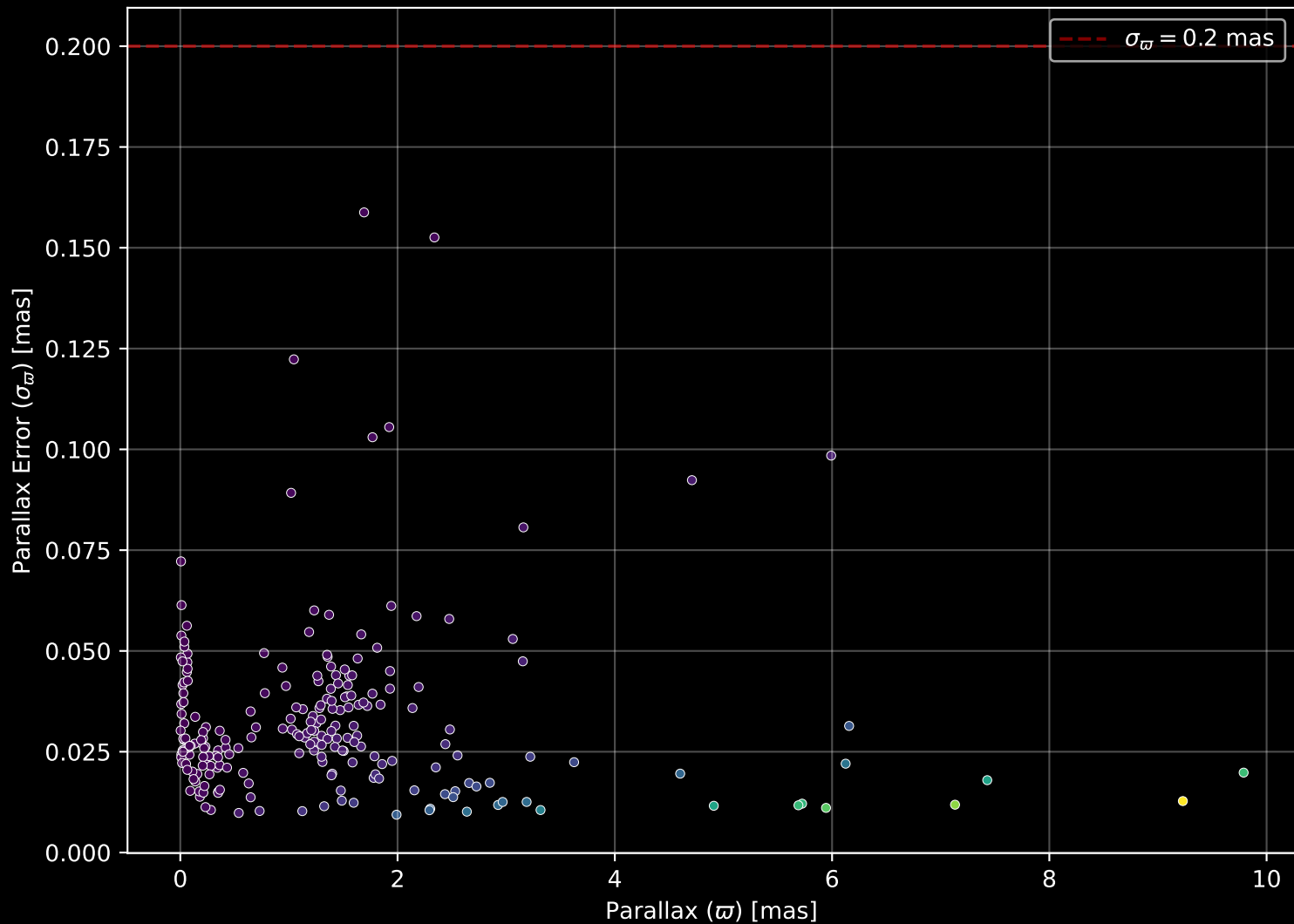
APOGEE DR17 Field: [293-37-C] Parallax Quality (n= 221)
