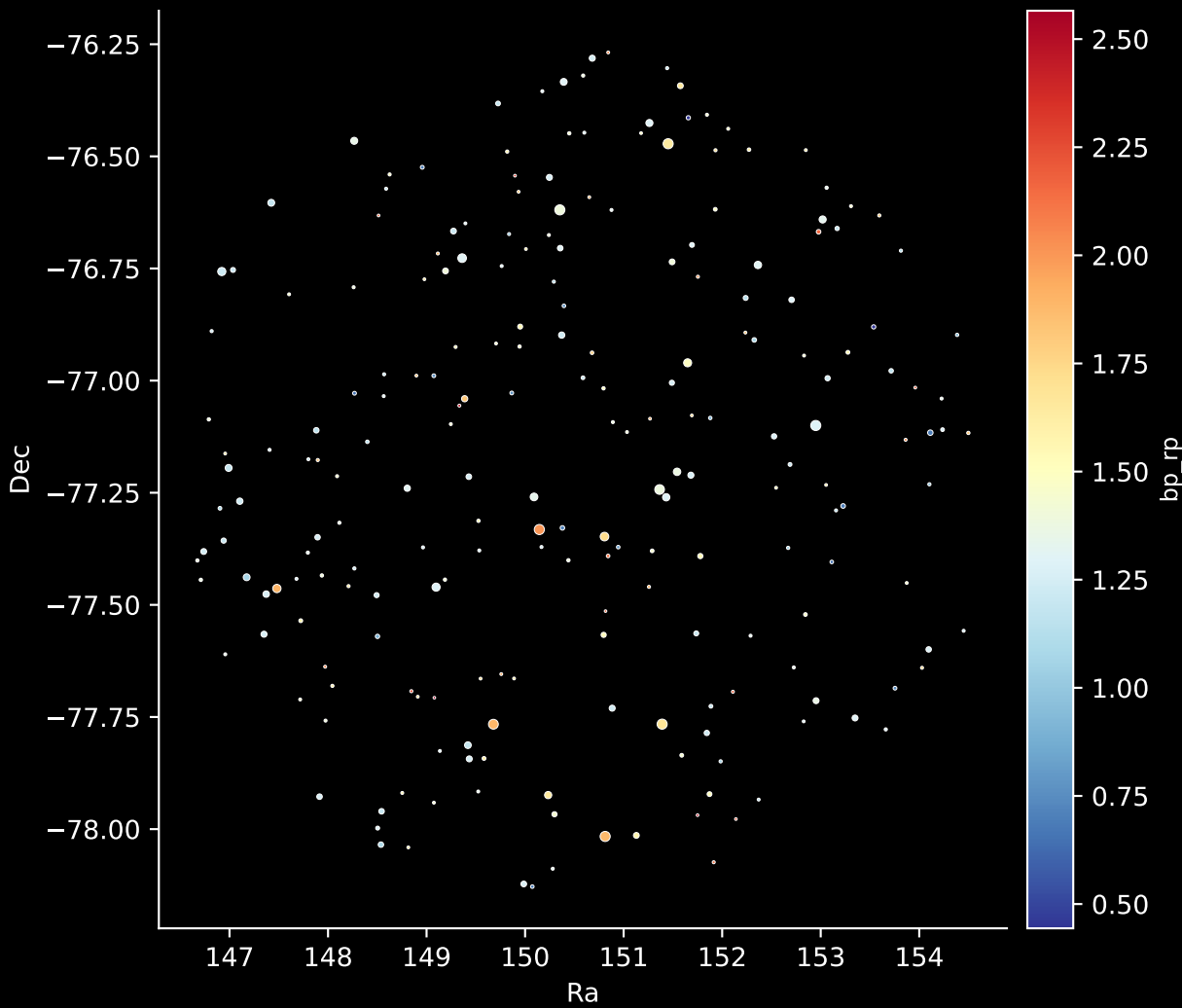
APOGEE DR17 Field: [293-37-C] Stars: 221
